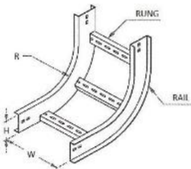
LIRI2 (I/R TYPE) LZRI2 (Z TYPE) LORI2 (O/R TYPE) 90DEG INSIDE RISER
