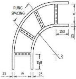
LIE2B (I/R TYPE) LZE2B (Z TYPE) LOE2B (O/R TYPE) 90DEG ELBOW (CURVE RADIUS)
