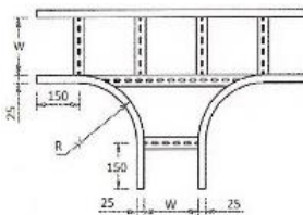
LIRI2 (I/R TYPE) LZRI2 (Z TYPE) LORI2 (O/R TYPE) 90DEG INSIDE RISER
