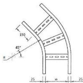
LIE1B (I/R TYPE) LZE1B (Z TYPE) LOE1B (O/R TYPE) 45DEG ELBOW (CURVE RADIUS)
