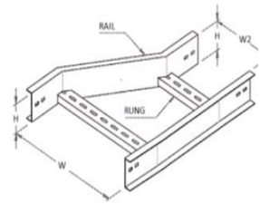
LIRRR (I/R TYPE) LZRRR (Z TYPE) LORRR (O/R TYPE) RIGHT-HAND REDUCER
