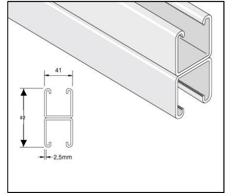
SLOTTED UNISTRUT UNISTSHDG41213M UNISTSHDG41216M
