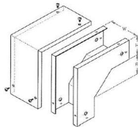
TKO2R 90EG OUTSIDE RISER
