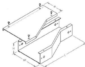
TKLRR LEFT HAND REDUCER
