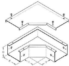
TKE2B 90DEG ELBOW
