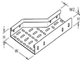
TFRRR RIGHT HAND REDUCER
