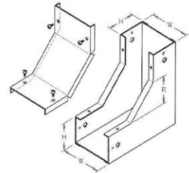
TKI2R 90DEG INSIDE RISER
