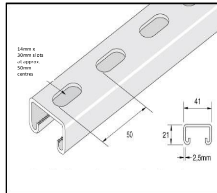
SLOTTED UNISTRUT UNISTSHDG41213M UNISTSHDG41216M
