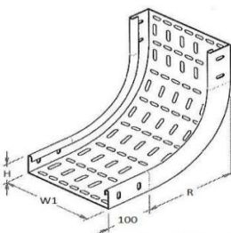
TFI2R 90DEG INSIDE RISER (CURVE RADIUS)
