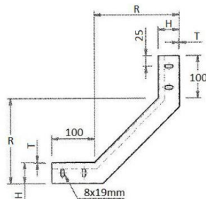
TFI2R 90DEG INSIDE RISER (STRAIGHT RADIUS)
