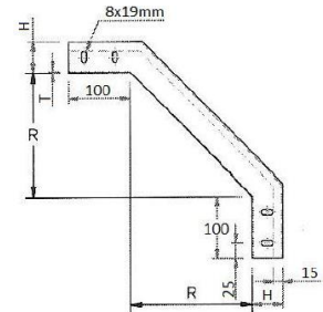
TFO2R 90DEG OUTSIDE RISER (STRAIGHT RADIUS)
