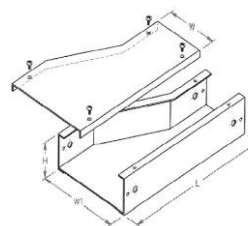
TKRRR RIGHT HAND REDUCER
