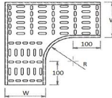
TFE2B 90DEG ELBOW (CURVE RADIUS)
