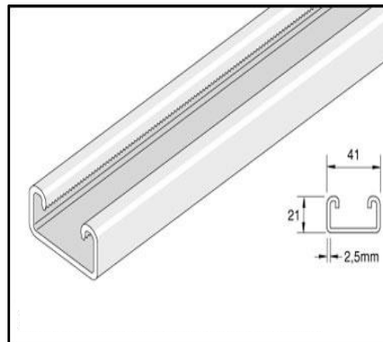
STRAIGHT UNISTRUT UNISTTHDG41213M UNISTTHDG41216M
